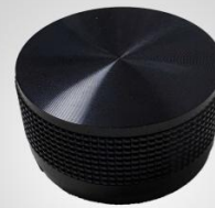
HJ-L136 Φ40*22mm
